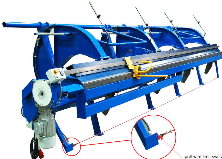
pull-wire limit switch
