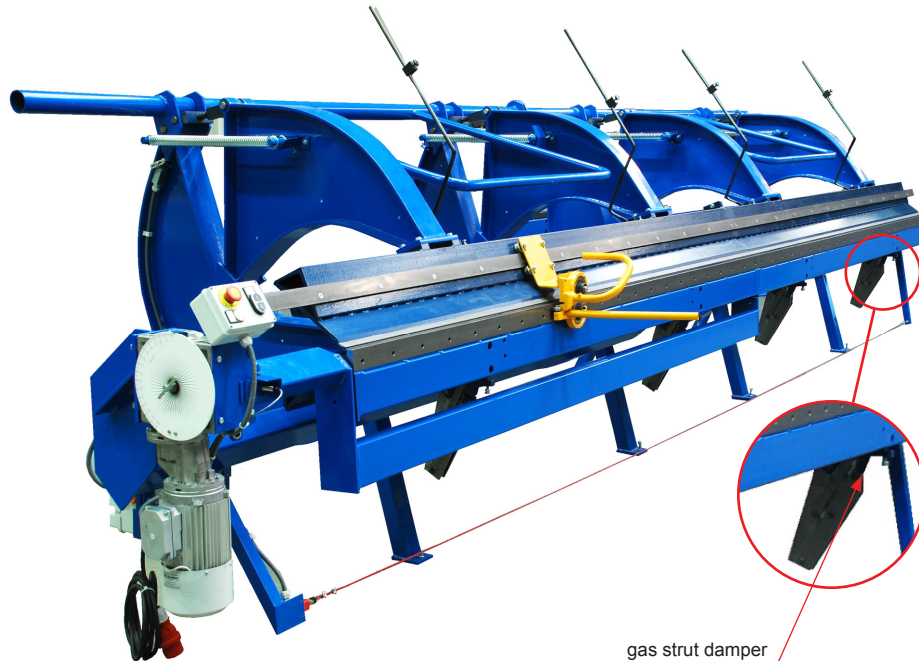
gas strut damper
