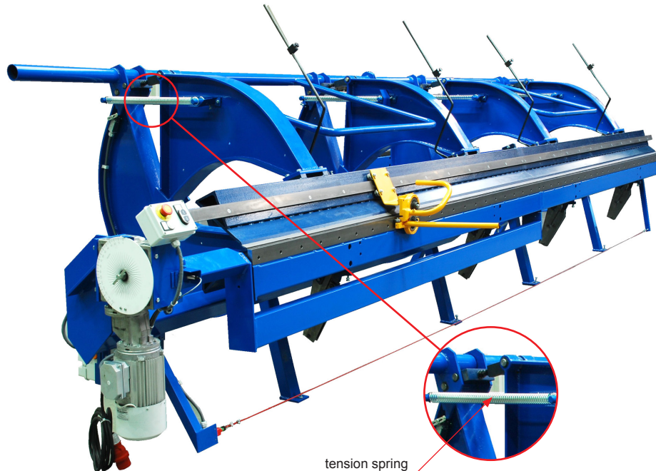
tension spring
