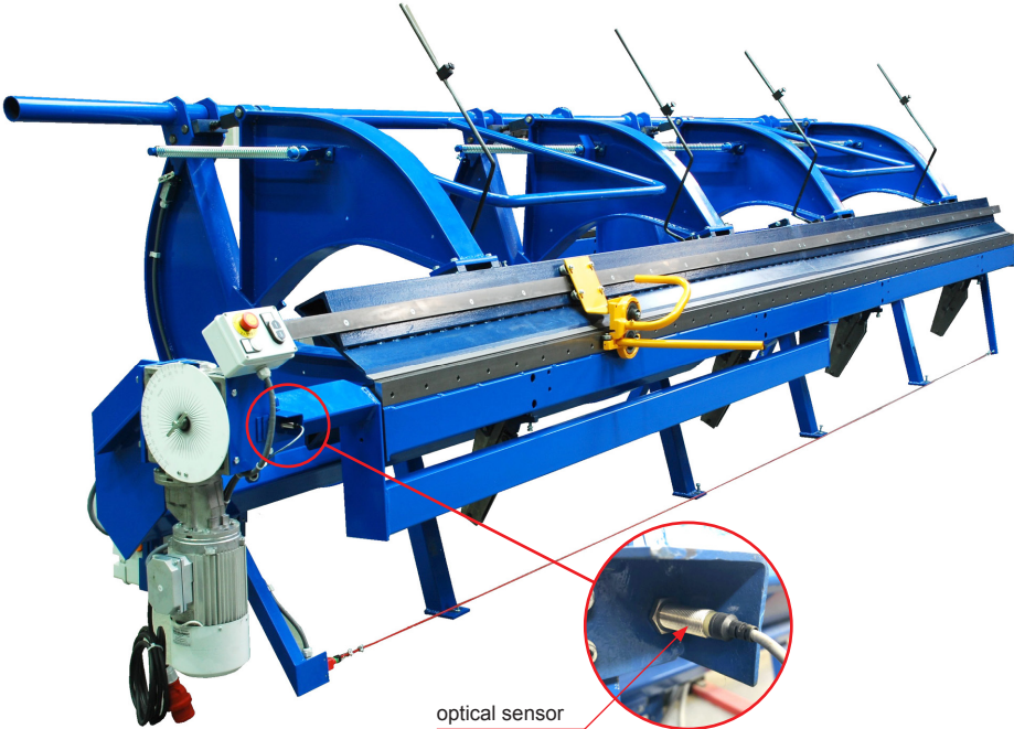
optical sensor
