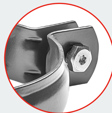
SLEEVE M10 STAINLESS STEEL SCREW M8x30 (Aluminium, Stainless steel)
