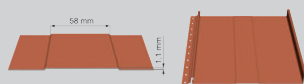
T58 – PRELIS 58 mm
