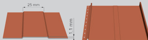
T25 – PRELIS 25 mm
